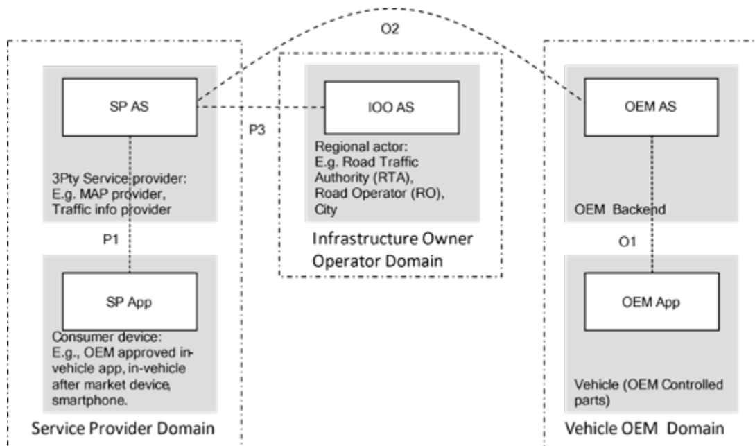
Figure 7: System architecture of traffic event information sharing UC – using O1 interface
