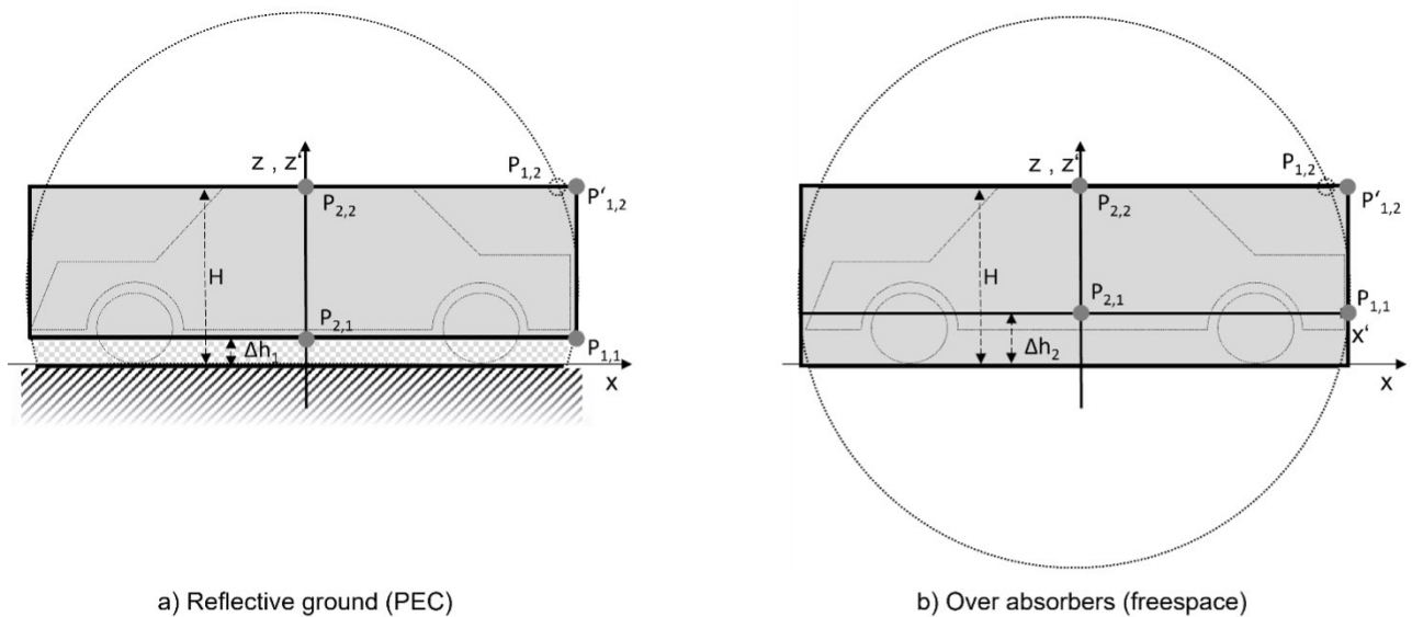
Figure 9: Alternative measurement positions based on cylindrical volume (vertical cut at y=0 )
