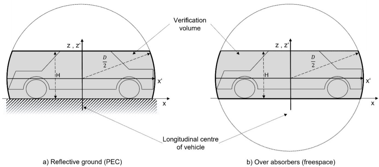
Figure 5: Size and orientation of the verification volume (side view)
