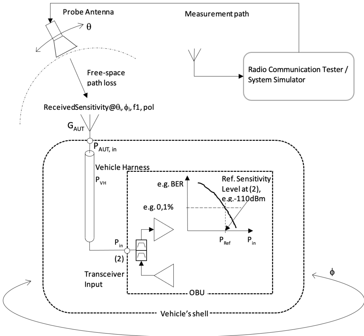
Figure 19: OTA measurement setup, radiated sensitivity
