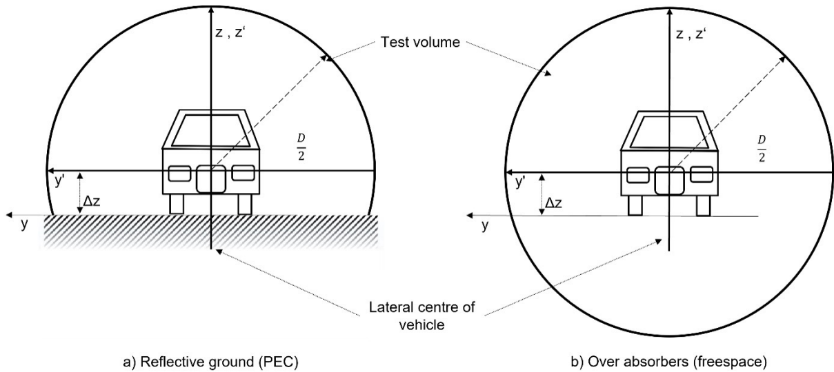
Figure 4: Size and Orientation of the measurement test volume (front view)
