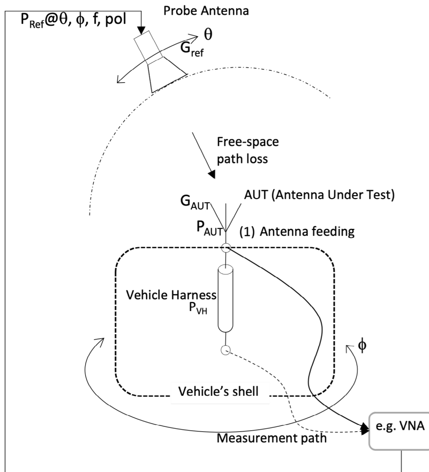
Figure 11: Antenna pattern measurement setup
