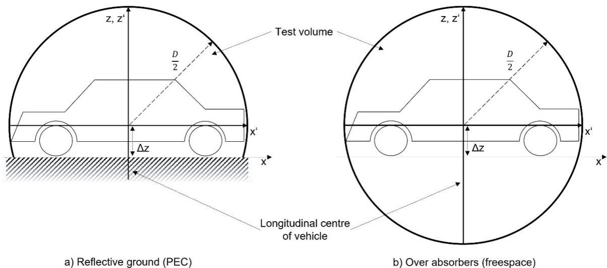
Figure 3: Size and orientation of the measurement test volume (side view)
