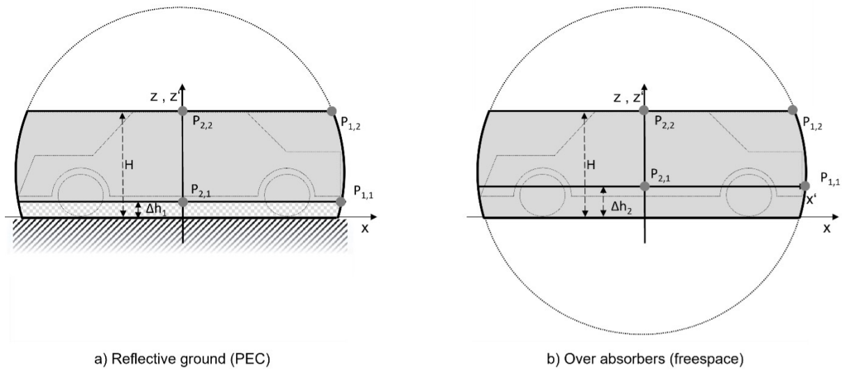
Figure 7: Measurement positions based on discretisation of the verification volume (vertical cut at y=0 )
