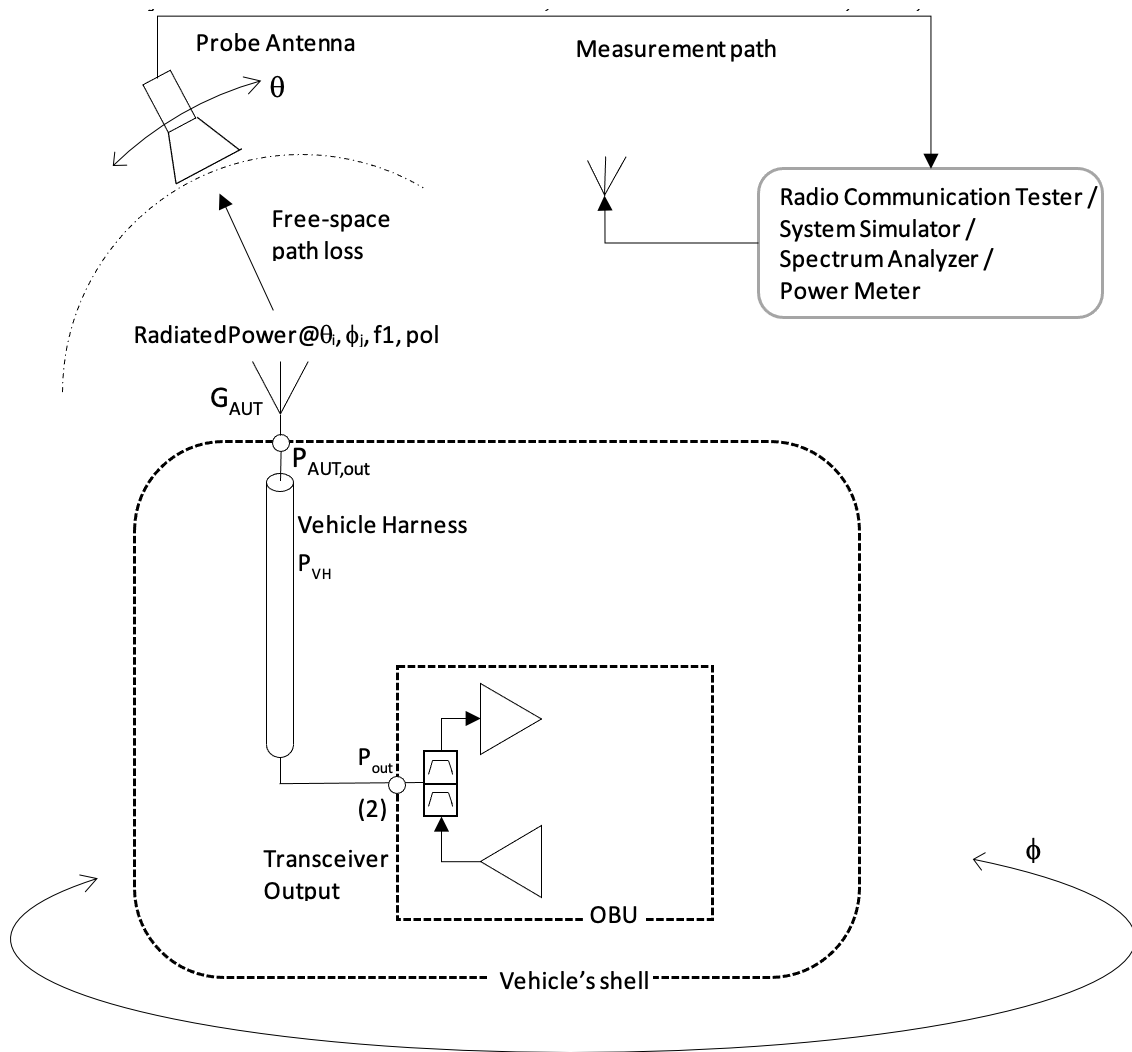
Figure 18: OTA measurement setup, radiated power
