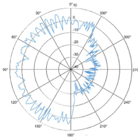
Figure 10: Example of an antenna radiation pattern [dB]
