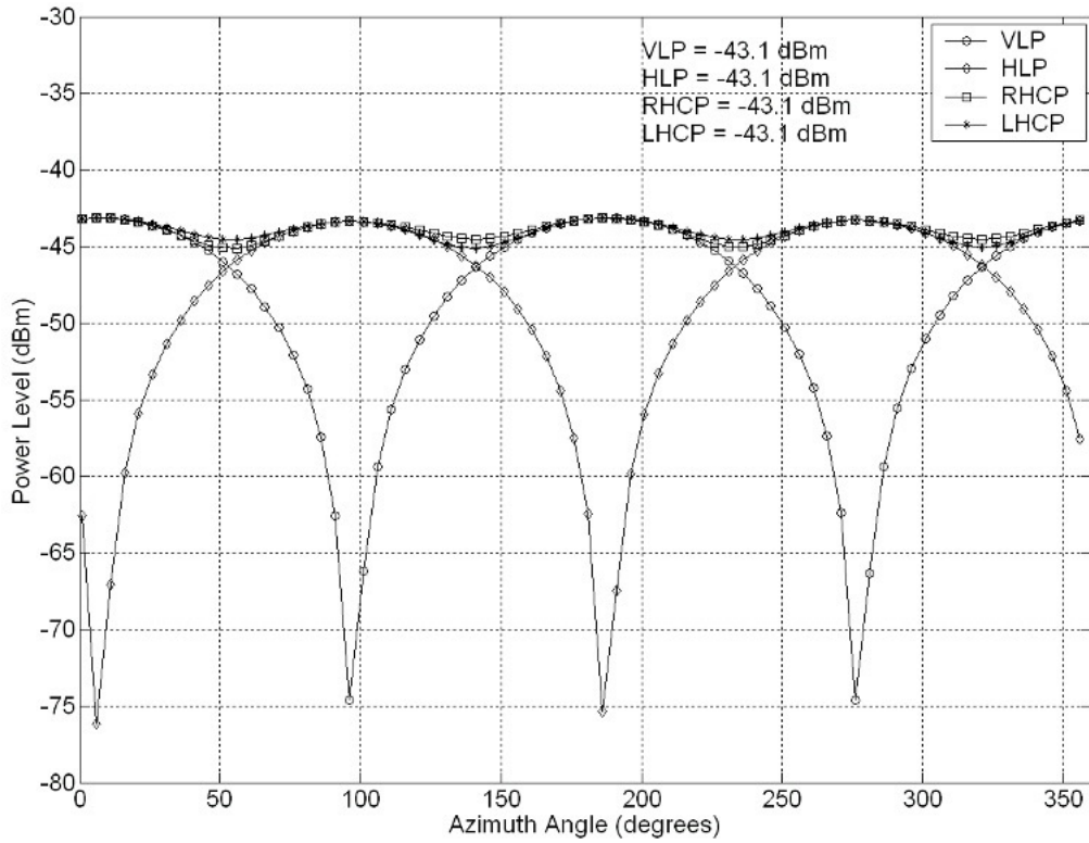
Figure 16: Ideally computed received power level response of a standard gain horn at boresight vs. azimuth angle for VLP, HLP, RHCP and LHCP
