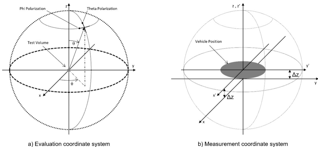
Figure 1: Coordinate systems and antenna polarisations
