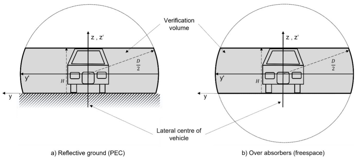
Figure 6: Size and orientation of the verification volume (front view)
