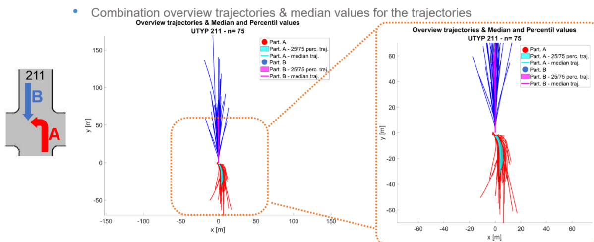
Figure 86: Trajectories of Left turn accident (211)
