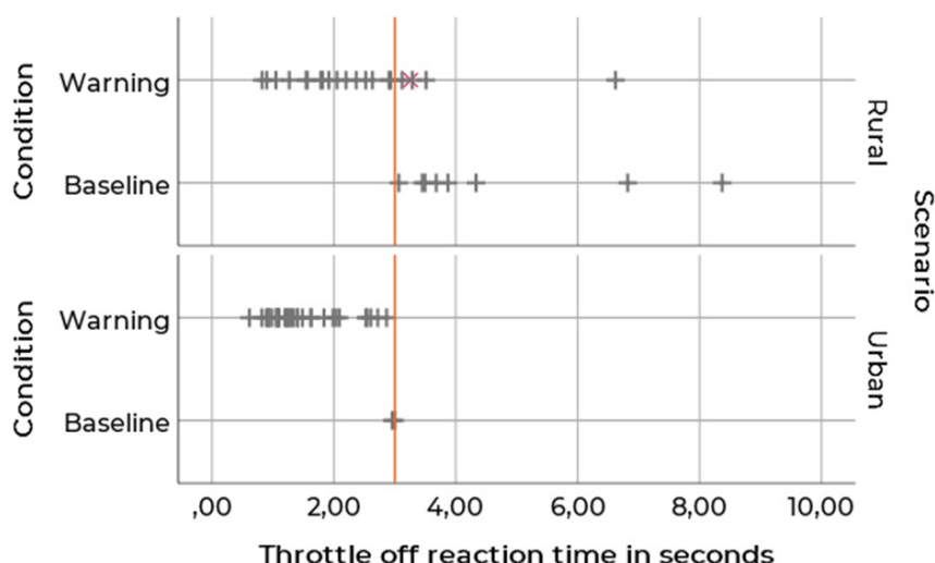
Figure 110: Riders' throttle off reaction times after the warning has been emitted for rural and urban scenarios. In warning and baseline (corresponding time section) condition, + indicates a single measurement, x indicates a reaction, where the rider stated to not have seen a warning, the orange vertical line indicates the point in time when the obstacle becomes visible and the warning disappears
