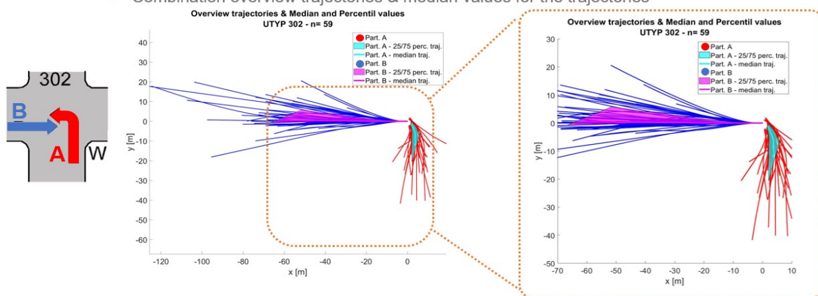
Figure 43: Trajectories of crossing traffic accident (302)
