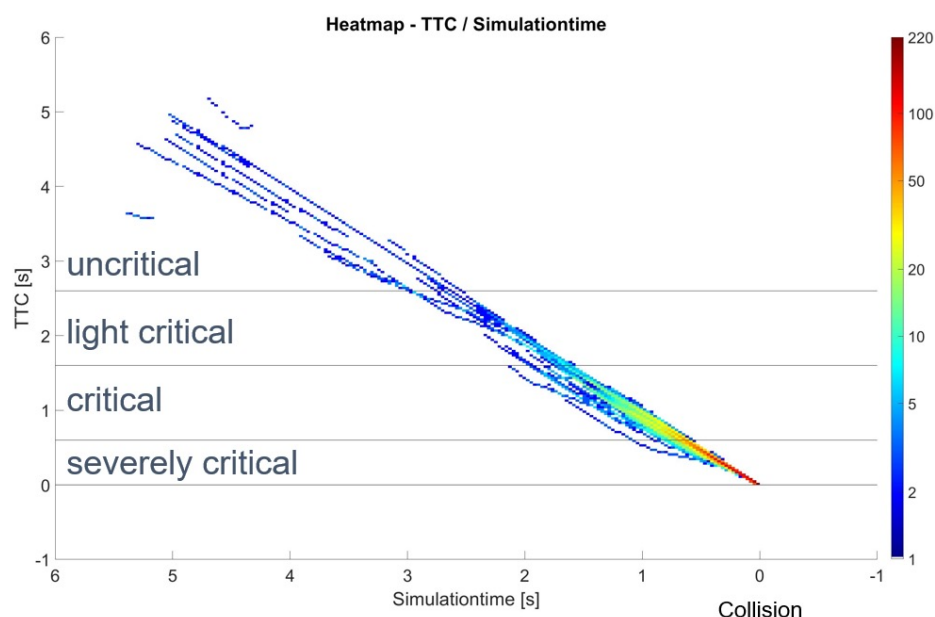
Figure 95: TTC calculation result for Left turn accident 211
