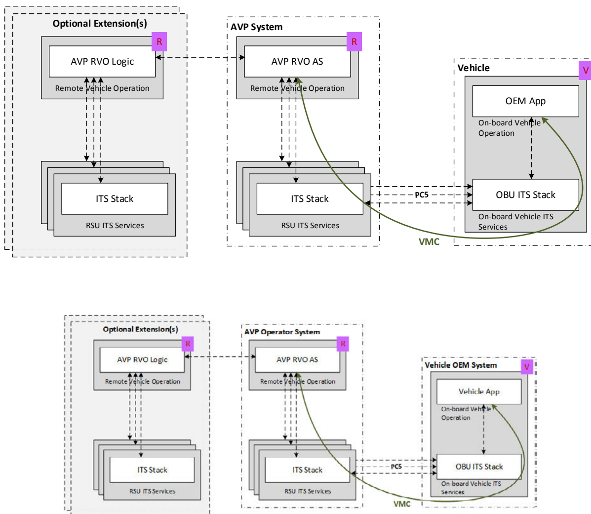
Figure 24: Split RSU/RVO architecture
