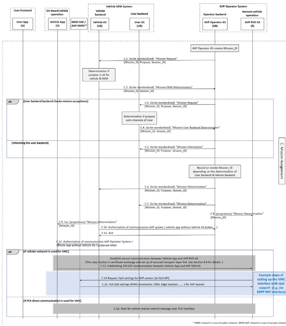
Figure 10: Communication sequence for 'mission assignment'
