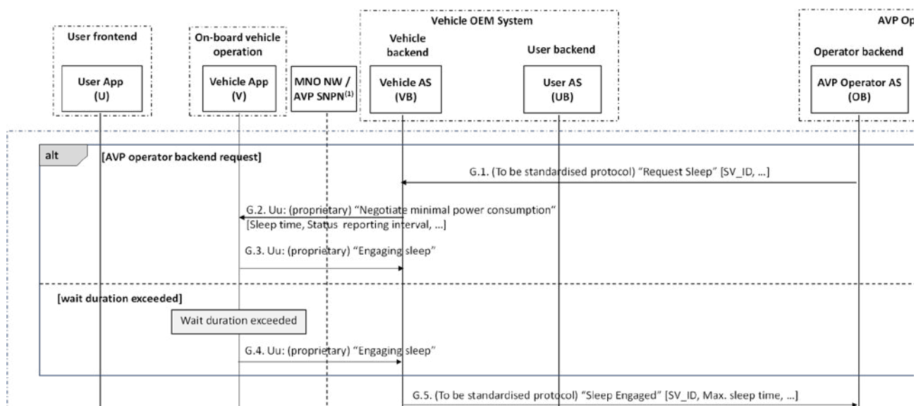
Figure 15: Communication sequence for 'sleep'
