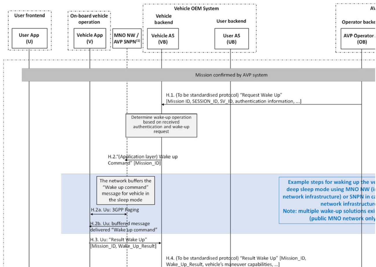
Figure 16: Communication sequence for 'wake-up'
