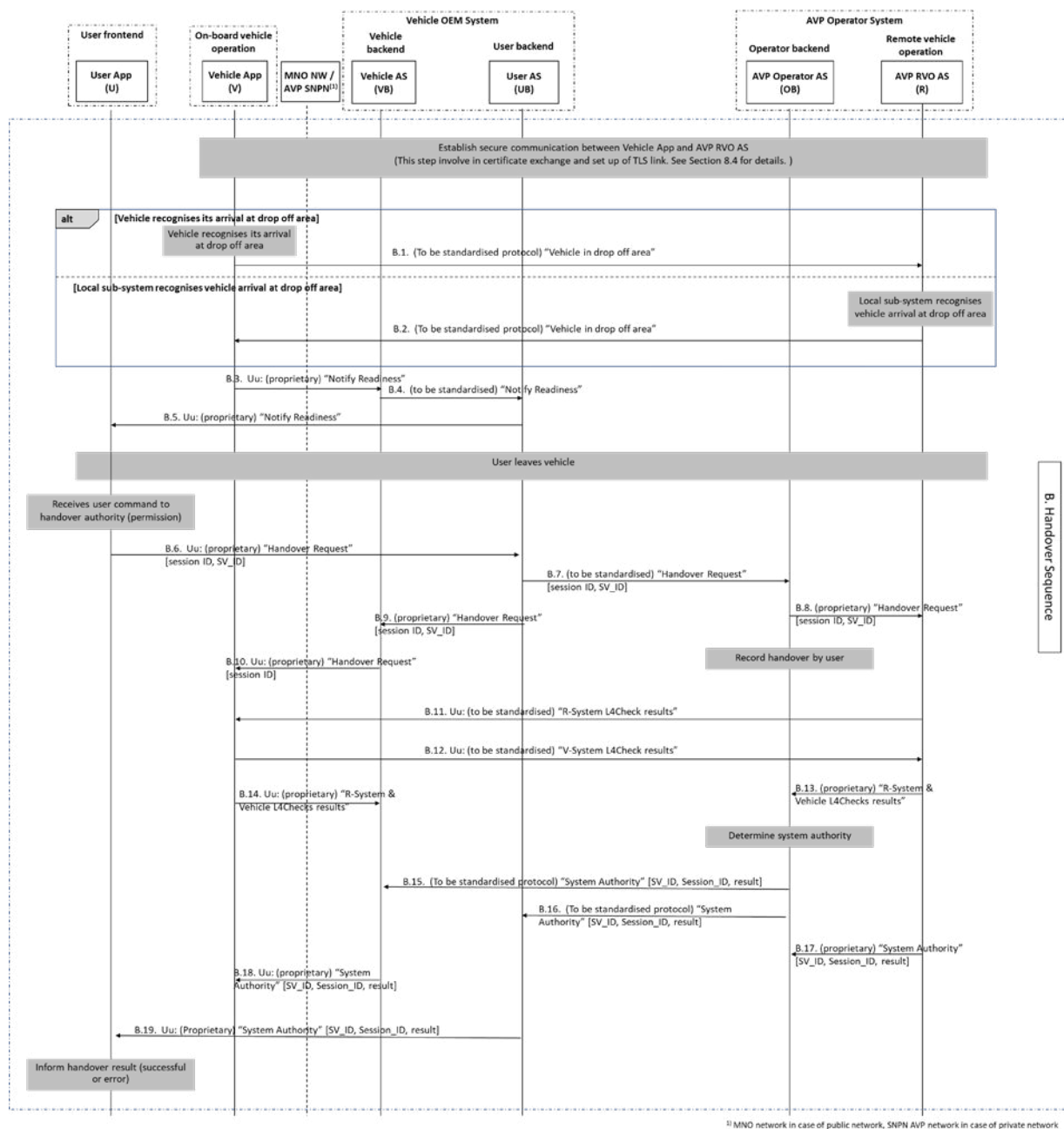
Figure 9: Communication sequence for 'handover'
