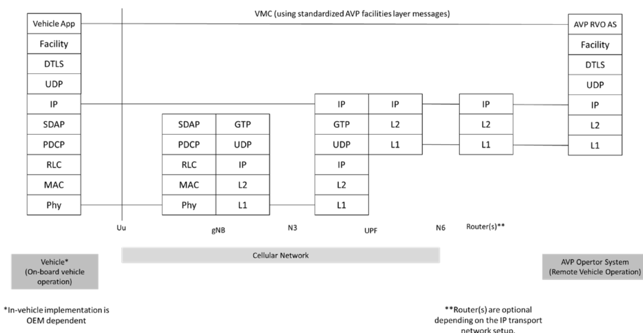
Figure 22: Example protocol stacks for vehicle motion control
