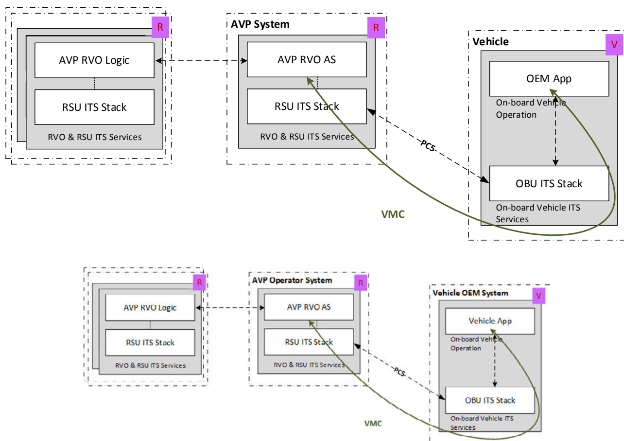
Figure 25: Co-located RVO-RSU architecture
