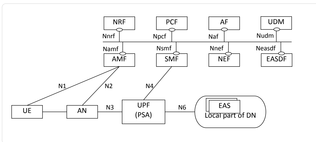
Figure 3: Addition of EASDF in 3GPP core network architecture
