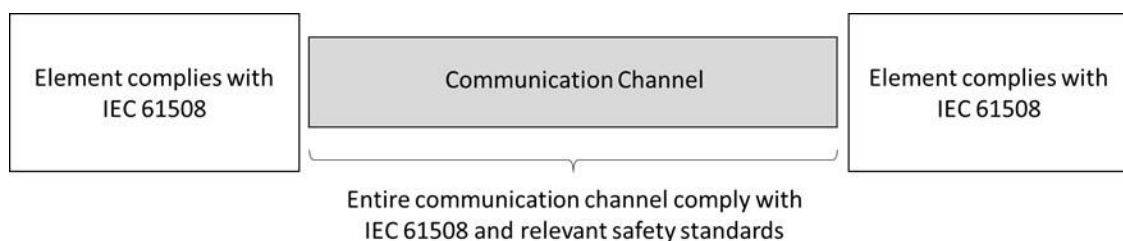
Figure 7-1: Closed channel
