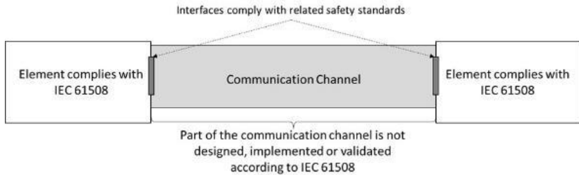
Figure 7-2: Open channel
